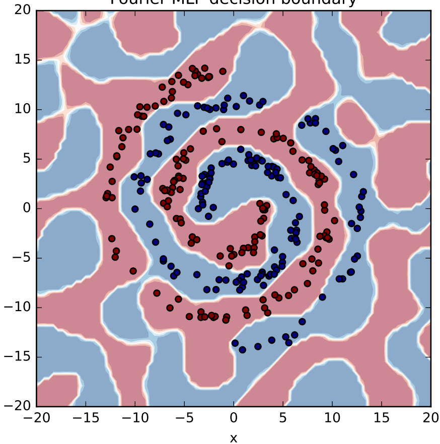
Fourier MLP decision boundary
